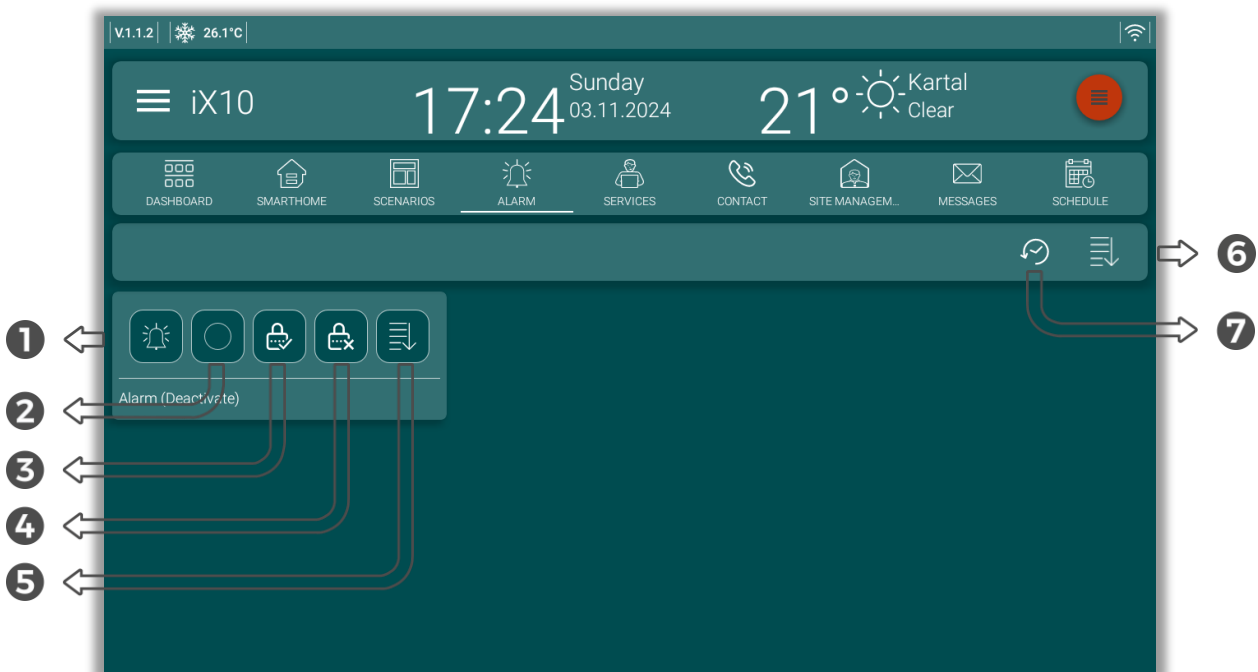
Fig. 22: Alarm Section
