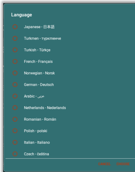
Fig. 68: Language List
