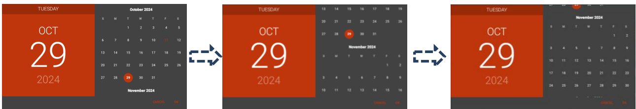
Fig. 72: Calendar List
