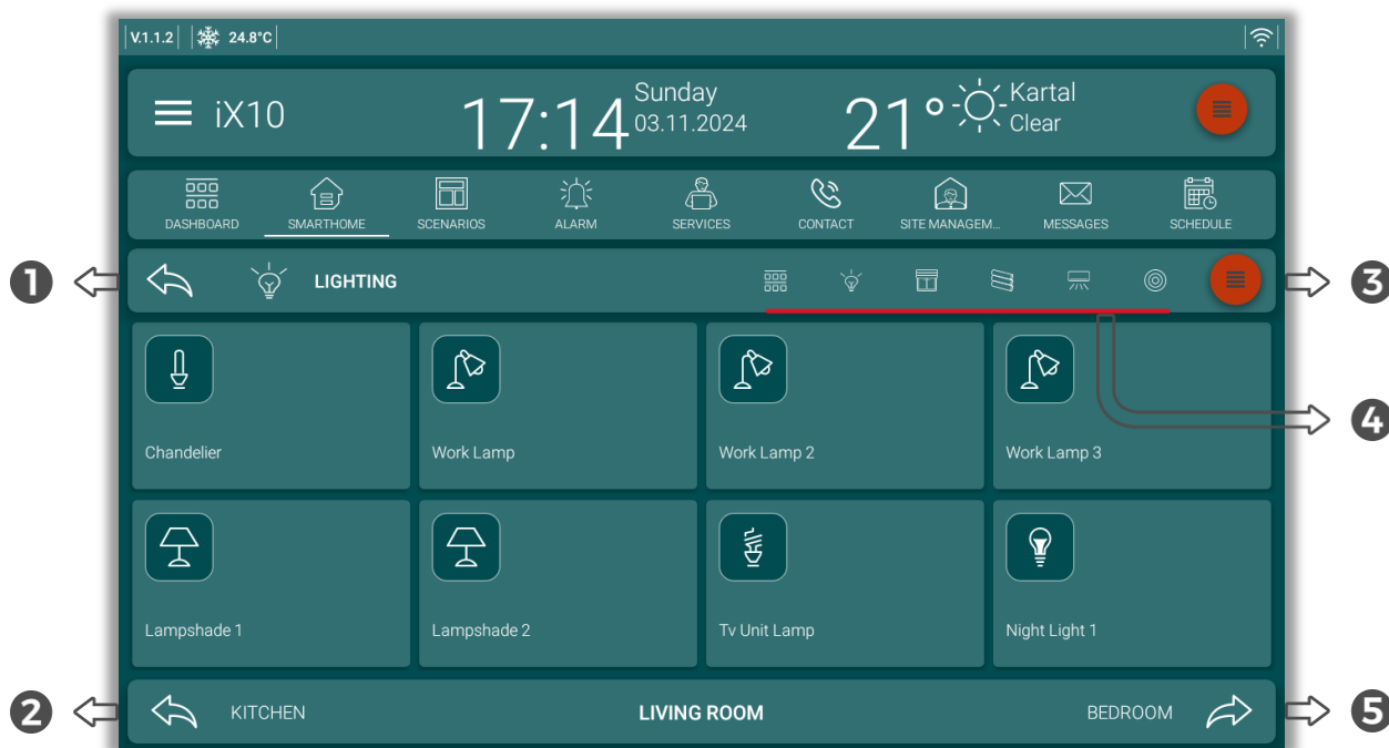
Fig. 10: Lighting Section
