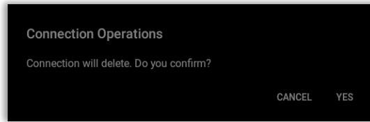
Fig. 61: Connections – Delete
