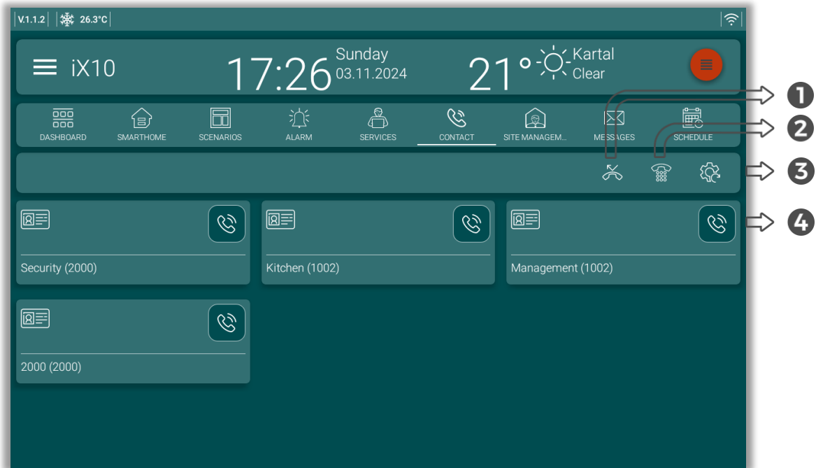
Fig. 29: Contact Section
