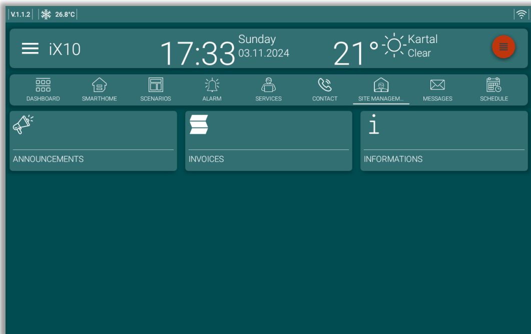
Fig. 32: Site Management
