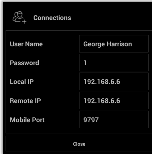
Fig. 62: Connections – Info
