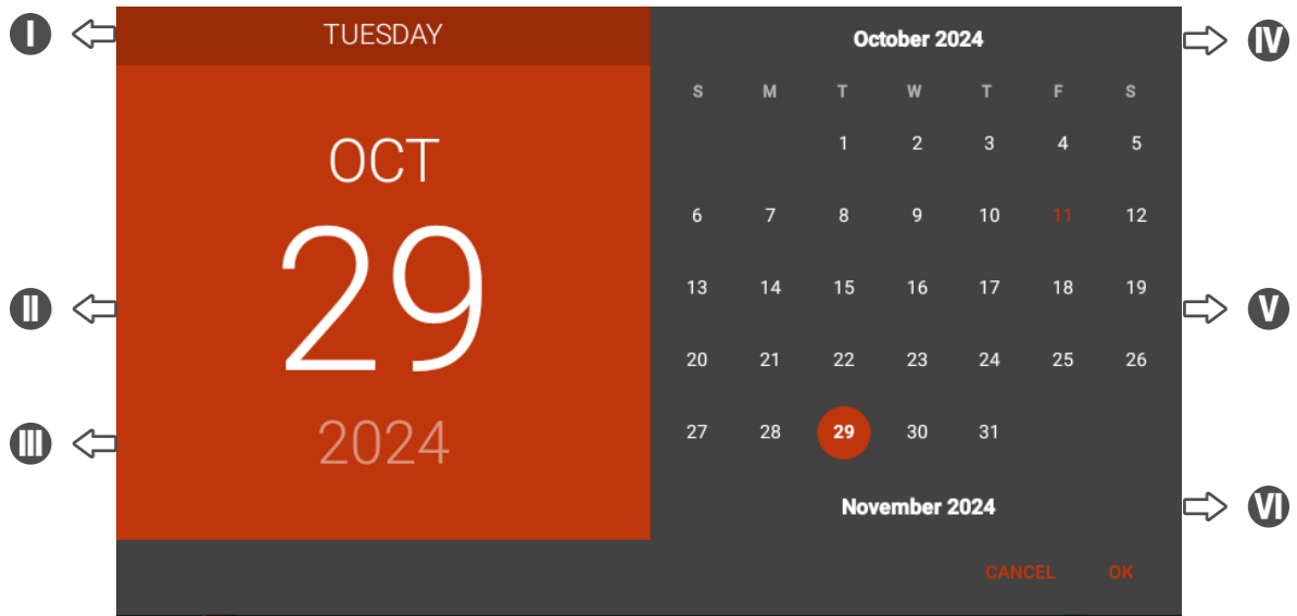
Fig. 70: Calendar Window
