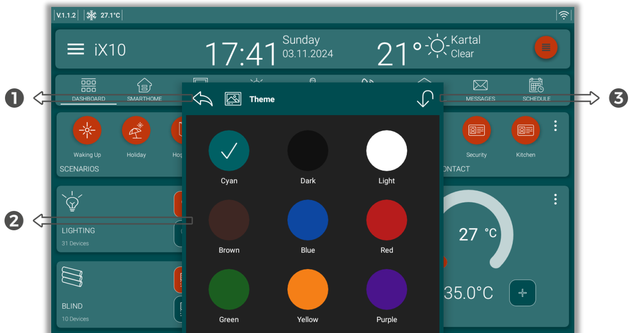
Fig. 83: Theme Section
