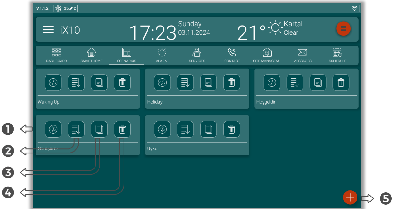
Fig. 16: Scenario Section
